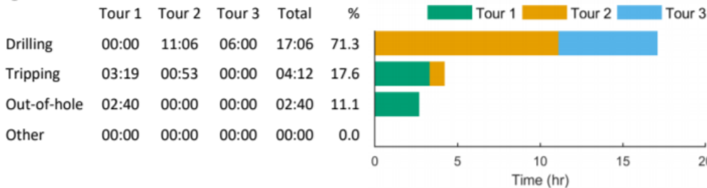
Rig State
