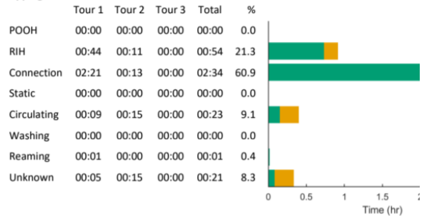
Tripping State
