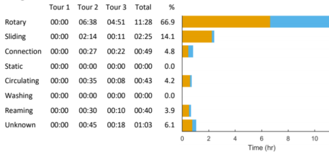
Drilling State
